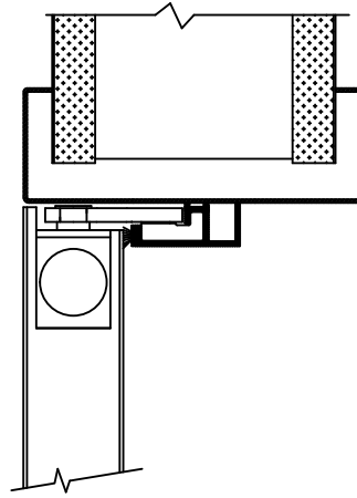
CASED HEAD DETAIL
