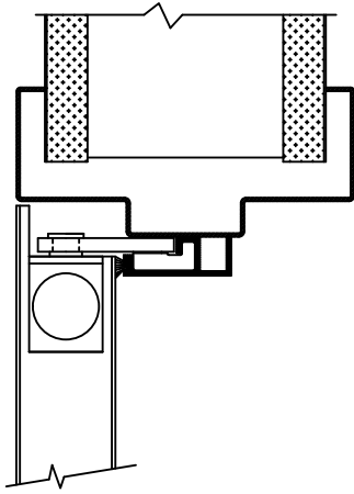
DOUBLE RABBET HEAD DETAIL
