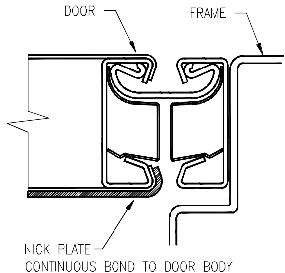
KICK PLATE SECTION
