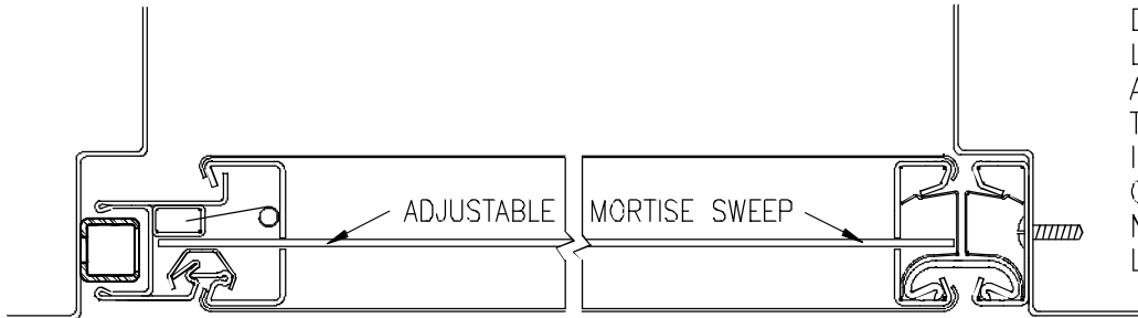
HORIZONTAL SECTION AT ADJUSTABLE MORTISE SWEEP
