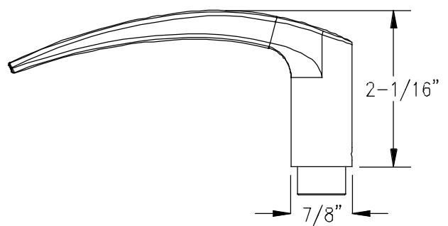
Q-84 LEVER DESIGN
