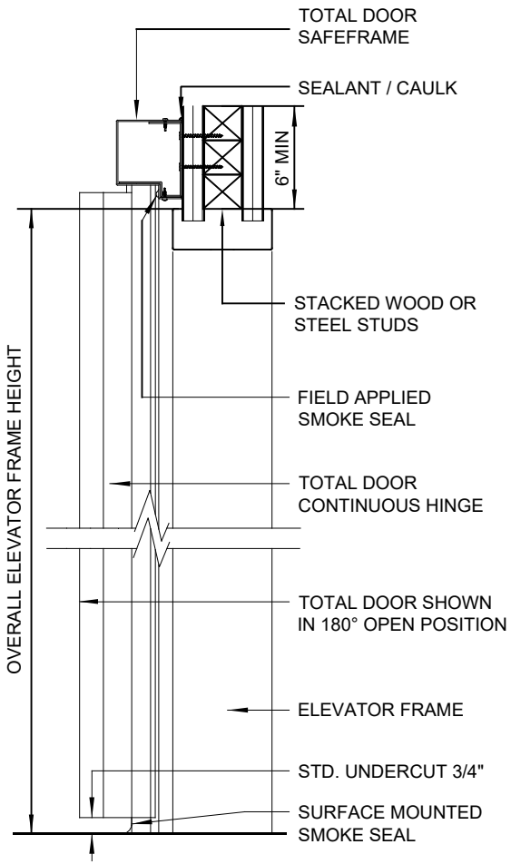
1 VERTICAL SECTION NOT TO SCALE
