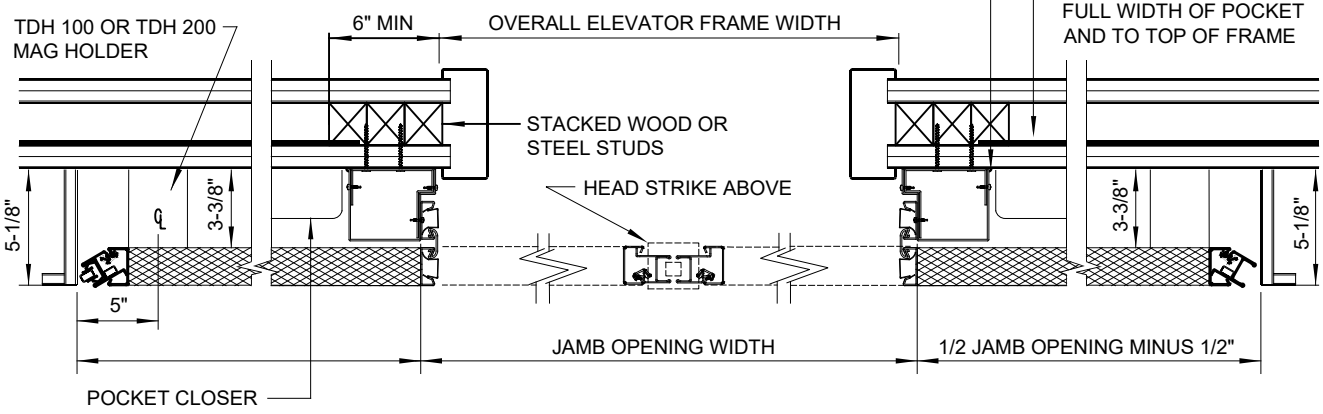
2 HORIZONTAL SECTION NOT TO SCALE
