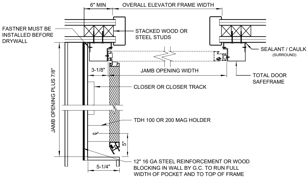
2 HORIZONTAL SECTION
