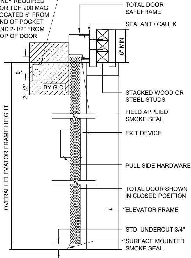
1 VERTICAL SECTION
