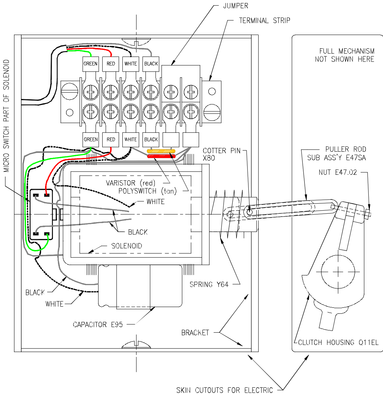
CUTAWAY VIEW - "E-UNL" MECH. (E19SA=EUN) - RH OR RR
