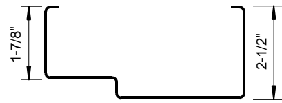
HEAD PROFILE
