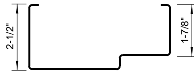
HEAD DETAIL
