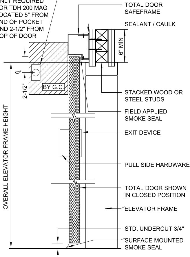
1 VERTICAL SECTION
