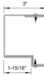
HEAD PROFILE
