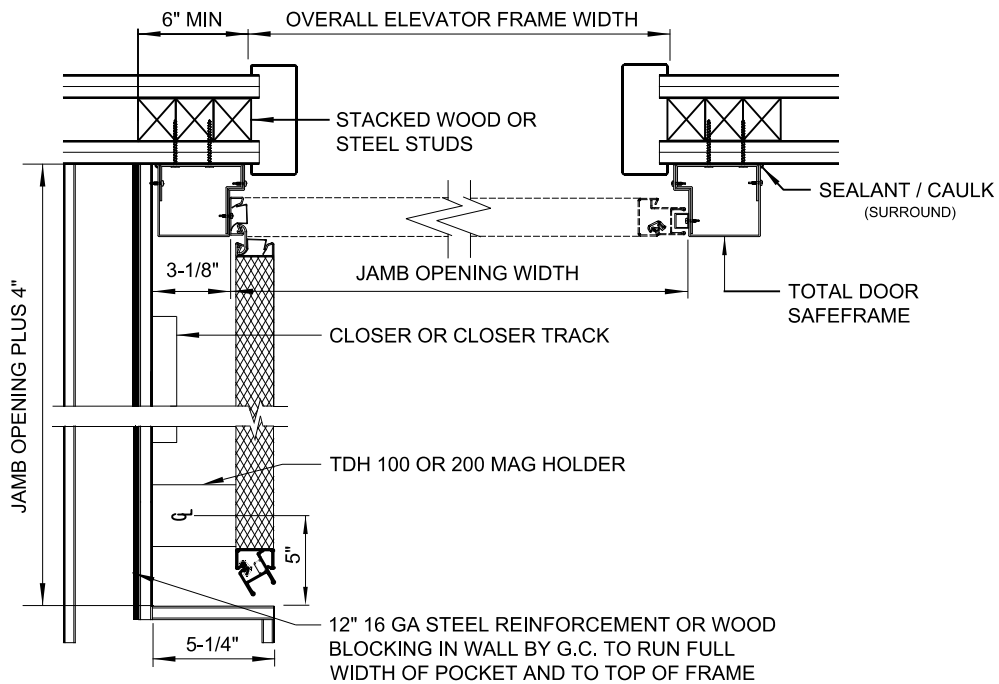
2 HORIZONTAL SECTION
