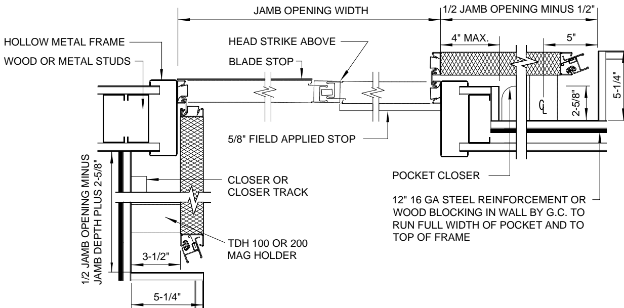
2 PLAN SECTION NOT TO SCALE
