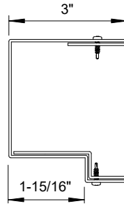
HEAD PROFILE
