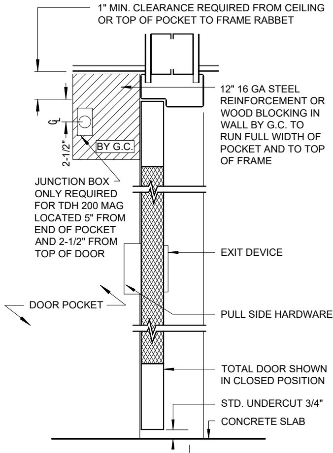
1 VERTICAL SECTION NOT TO SCALE
