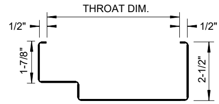
HEAD PROFILE
