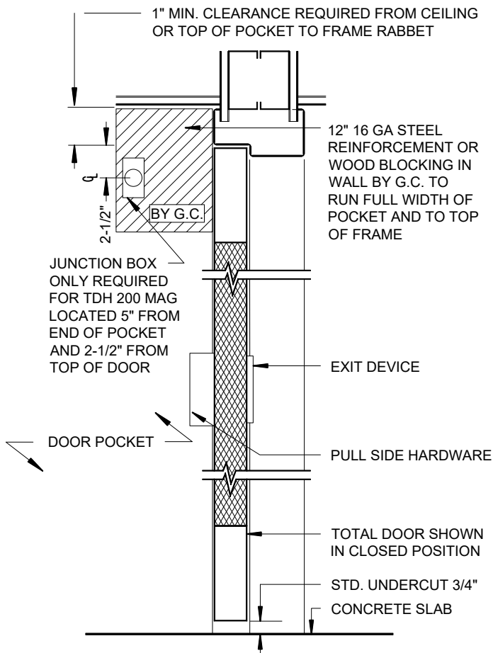
1 VERTICAL SECTION NOT TO SCALE
