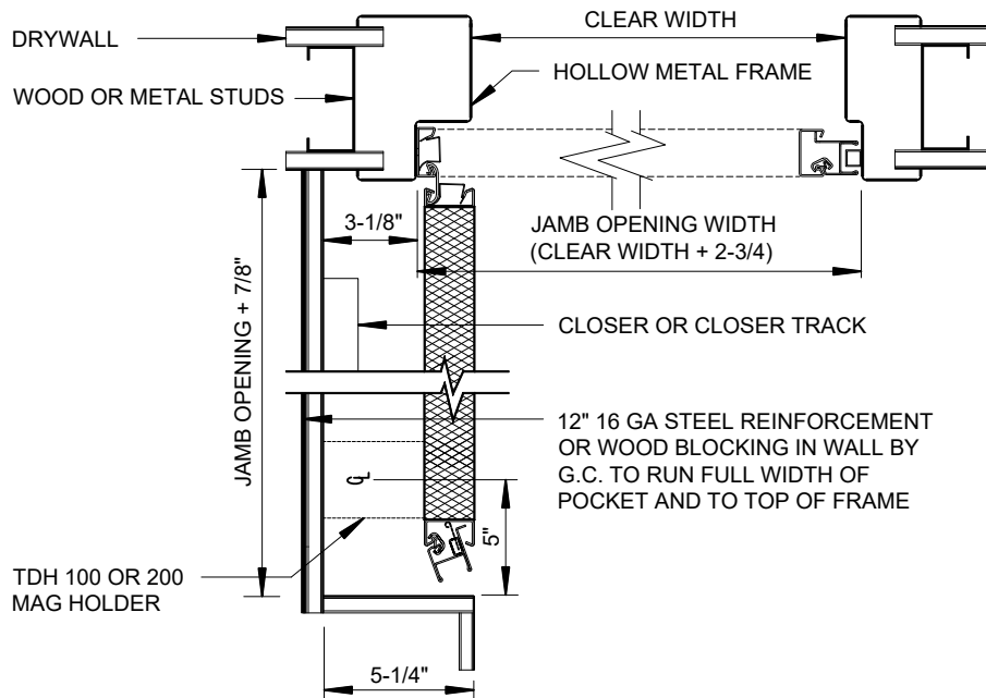
2 HORIZONTAL SECTION NOT TO SCALE
